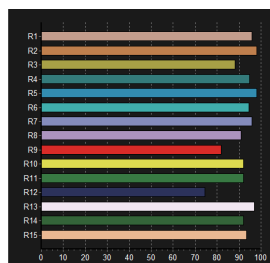
White 4000° CRI 95
