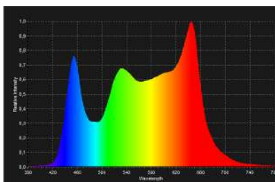
Curva White 4000°
