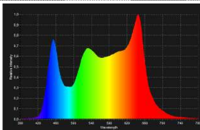
Curva White 4000°
